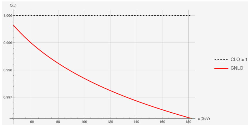
Figure 4: Evolution of the NLO WC with the scale \mu .
